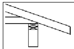
STANDARD HEEL TRUSS W/PLUM END CUT
